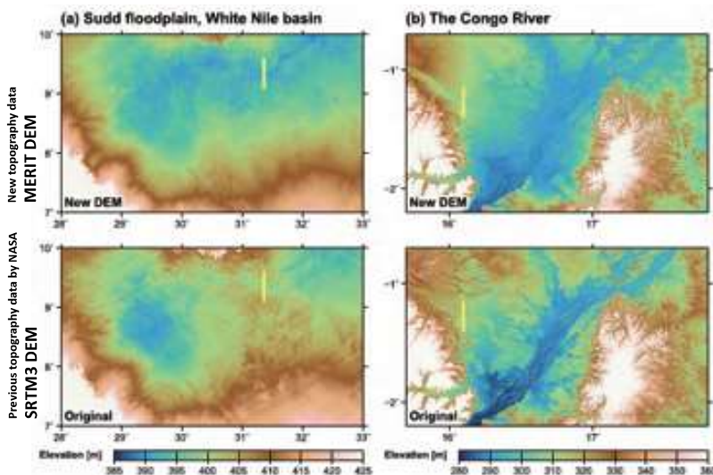
MERIT DEM: A precise topography by multi-component error removal High accuracy topography map was developed by combining multiple satellite data and removing multiple error components. Now widely used in various research fields.
