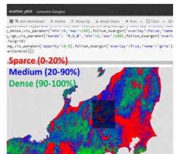
Analysis of global forest structure maps
